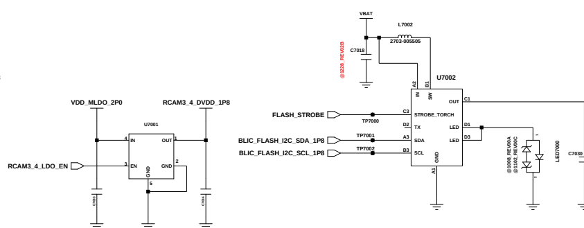
FLASH DRIVER
