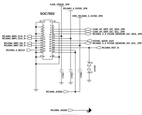
RCAM4_2M_MACRO (24PIN)_GC02M1
